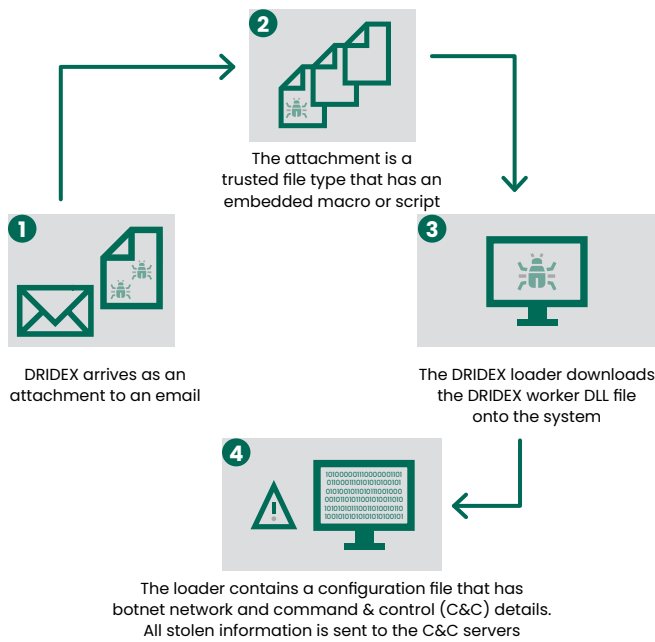
Figure 1: Ransomware through DRIDEX malware
