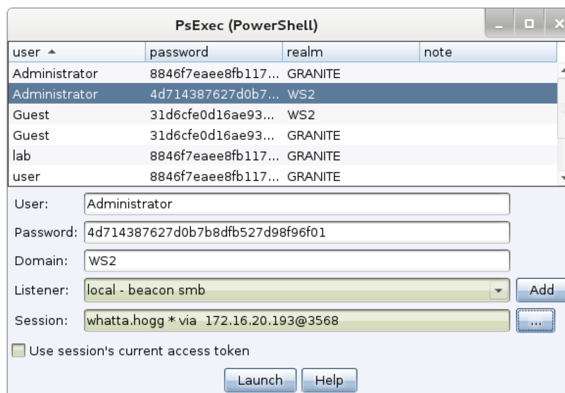
Figure 33. Lateral Movement Dialog
