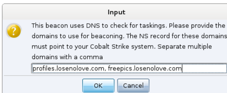
Figure 21. Configure DNS Beacon Domains
