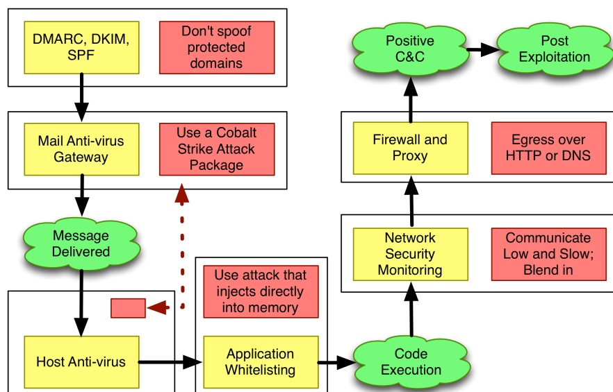
Figure 1. The Path to Post Exploitation
