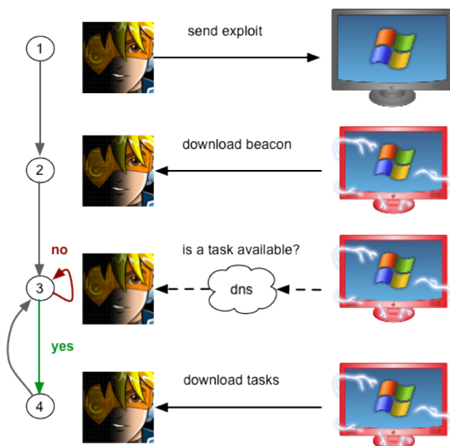
Figure 20. Hybrid HTTP and DNS Beacon in action
