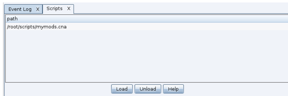
Figure 8. Script Manager
