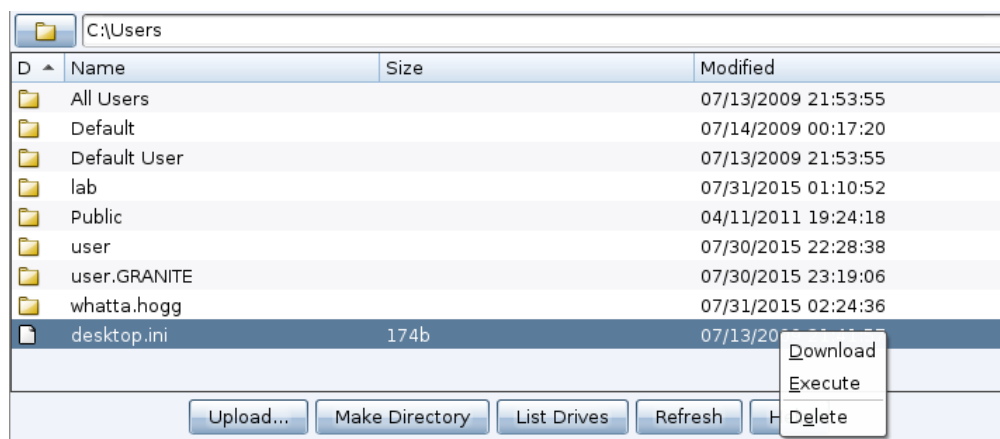
Figure 30. File Browser
