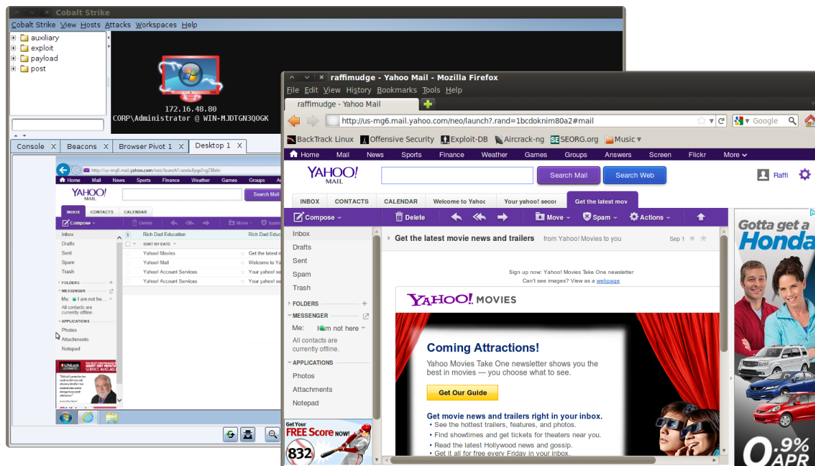
Figure 34. Browser Pivoting in Action
