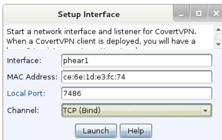
Figure 39. Setup a Covert VPN Interface
