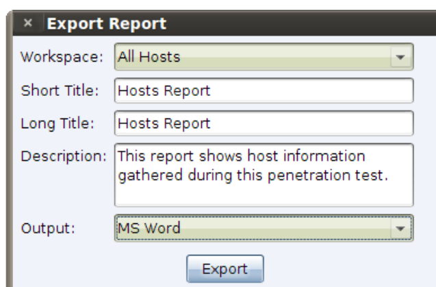
Figure 40. Export Report Dialog
