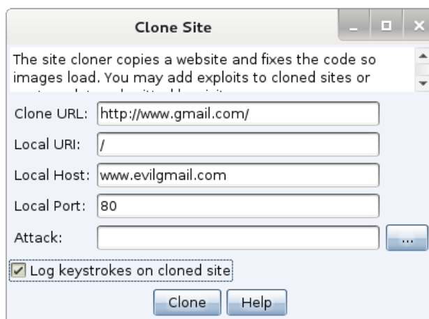
Figure 23. Website Clone Tool
