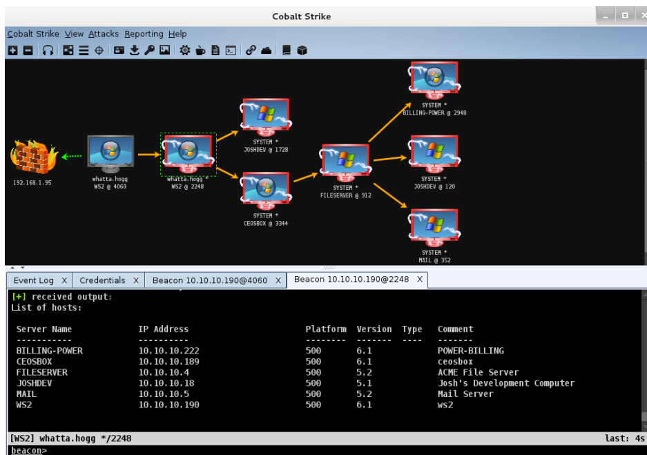
Figure 9. Cobalt Strike User Interface
