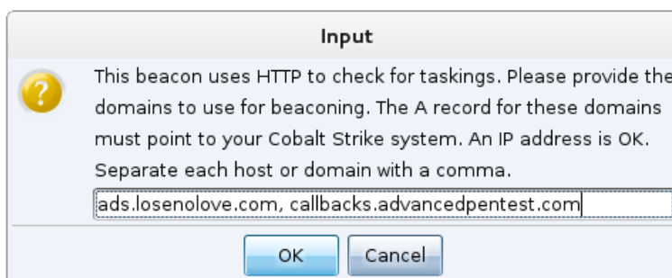
Figure 19. Configure Beacon Domains
