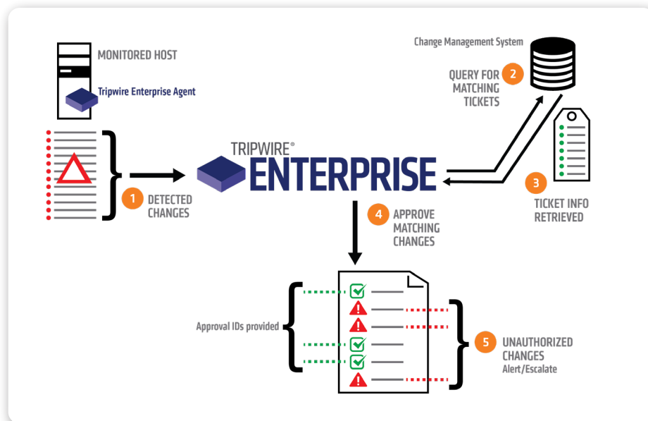
Fig. 1 Tripwire Enterprise Integration Framework automates system integrations with Service Desk products like ServiceNow, Remedy, Cherwell and others, for facilitating greater workflow efficiencies within IT security and operations.
